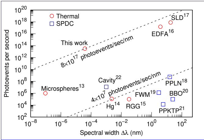
FIG. 1. Spectral densities of thermal and SPDC light sources based on: Microspheres[26] – suspension of microspheres, Hg[24, 27] – Mercury discharge lamp, RGG[13, 28] – rotating ground glass, EDFA[29] – Erbium-doped fiber amplifier, SLD[30] – superluminescent diode, PPLN[31] – periodically poled Lithium Niobate, FWM[32] – four-wave mixing, BBO[33] – Beta-Barium Borate, PPKTP[34] – periodically poled Potassium Titanyl Phosphate, Cavity[35] – enhancement by microring resonator.
