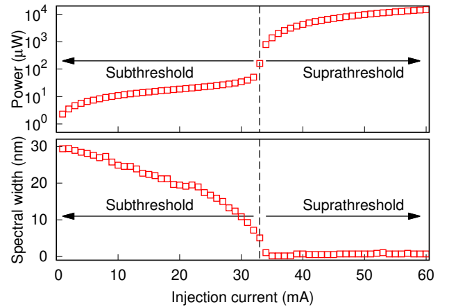
FIG. 2. Output power and spectral width \Delta\lambda of a laser diode as a function of its injection current to determine the lasing threshold.
