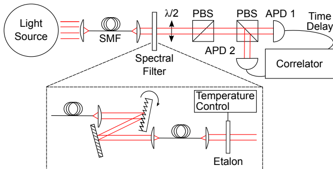
FIG. 1.— Setup to determine the temporal correlation g^{(2)}(\tau) for wide-band thermal light. The initial spectrum gets filtered to a narrow optical bandwidth such that the temporal decay of the second order correlation function can be observed with conventional single photon detectors in a Hanbury-Brown-Twiss experiment. We employ a combination of a grating and a temperature-tuned etalon as a spectral filter, and ensure spatial coherence in the setup by using single mode optical fibers (SMF).
