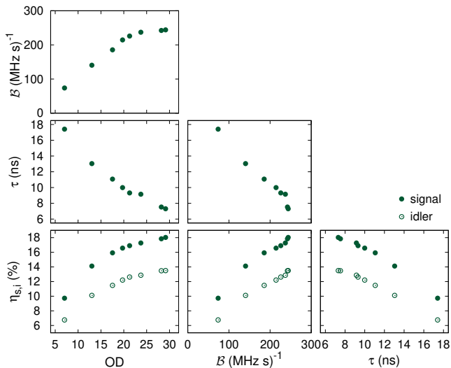
FIG. 16: Summary of the effect of optical density OD on heralding efficiencies \eta_{s,i} , coherence time \tau , and spectral brightness \mathcal{B} . Other parameters: P_{776} = 15 mW, P_{780} = 300 \mu W, \Delta = -60 MHz, \delta = 12 MHz.
