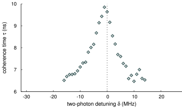
FIG. 13: Coherence time as function of detuning. Other parameters: P_{776} = 15 mW, P_{780} = 450 \mu W, \Delta = -60 MHz, OD = 29. The dotted line indicates \delta = 0 .
