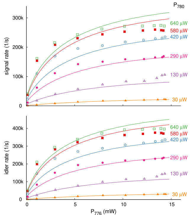
FIG. 6: Single rates for the signal (top) and idler (bottom) as a function of pump power at 776 nm ( P_{776} ) for different pump powers at 780 nm. The vertical error bar on each point is smaller than the size of the data points. Other parameters: OD = 29 , \Delta = -60 MHz, \delta = 3 MHz. The solid lines are numerical fits with Eq. 3.
