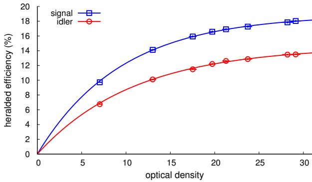
FIG. 5: Heralding efficiency for signal and idler modes as a function of the optical density. The solid lines are fits of Eq. 12 with \eta_{0s} = 0.190 \pm 0.001 and OD_{0s} = 9.7 \pm 0.1 , and \eta_{0i} = 0.150 \pm 0.001 and OD_{0i} = 11.3 \pm 0.2 . Other parameters: P_{776} = 15 mW, P_{780} = 300 \mu W, \Delta = -60 MHz, \delta = 12 MHz.
