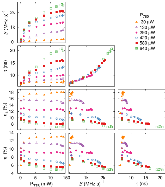
FIG. 15: Summary of the effect of pump powers P_1 and P_1 on heralding efficiencies \eta_{s,i} , coherence time \tau , and spectral brightness B . Other parameters: OD=29, \Delta = -60 MHz, \delta = 3 MHz.
