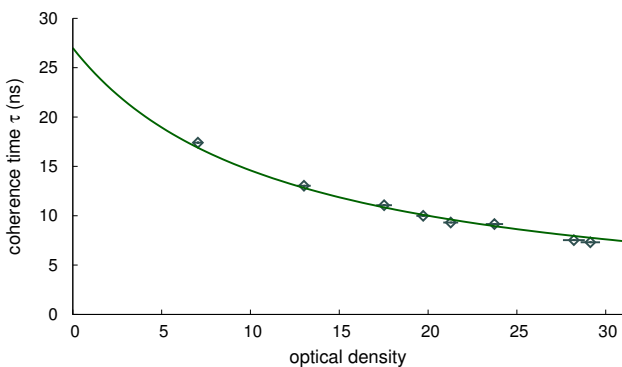
FIG. 3: Coherence time of the photon pair as a function of the optical density (OD) of the atomic cloud. The solid line is obtained by fitting Eq. 11, obtaining \mu = 0.0827 \pm 0.002 . Other parameters: P_{776} = 15 \text{ mW} , P_{780} = 300 \mu\text{W} , \Delta = -60 \text{ MHz} , \delta = 12 \text{ MHz} .
