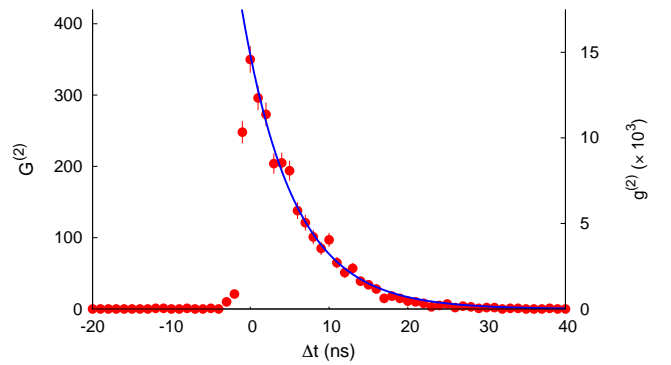
FIG. 2: Histogram of coincidence events G^{(2)}(\Delta t) (left vertical axis) and the normalized second order correlation g^{(2)}(\Delta t) (right vertical axis) as a function of the time difference between the detection of signal and idler photons for a total integration time of 42 s. Pump powers: P_{780} = 450 \mu\text{W} and P_{776} = 3 \text{ mW} , detunings \Delta = -60 \text{ MHz} and \delta = 12 \text{ MHz} . The solid line is a fit to the model described by Eq. 6, giving a value of \tau = 6.52 \pm 0.04 \text{ ns} .
