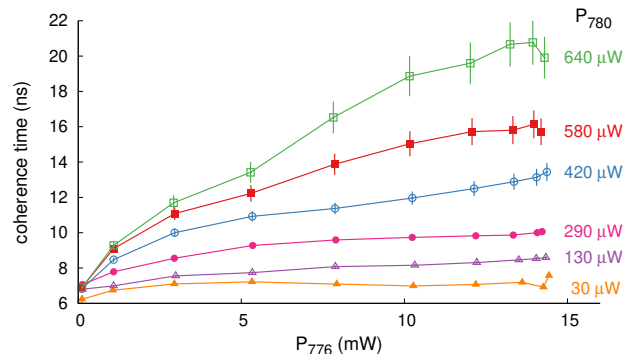
FIG. 12: Coherence time as function of pump powers. Other parameters: \text{OD} = 29 , \Delta = -60 MHz, \delta = 3 MHz.
