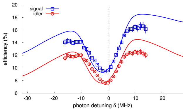
FIG. 10: Efficiency of the source as a function of the detuning from the two photon resonance \delta . Other parameters: P_{776} = 15 mW, P_{780} = 450 \mu\text{W} , \Delta = -60 MHz, \text{OD}=29 . The solid lines are fits with Eq. 5, the dotted line indicates \delta = 0 .
