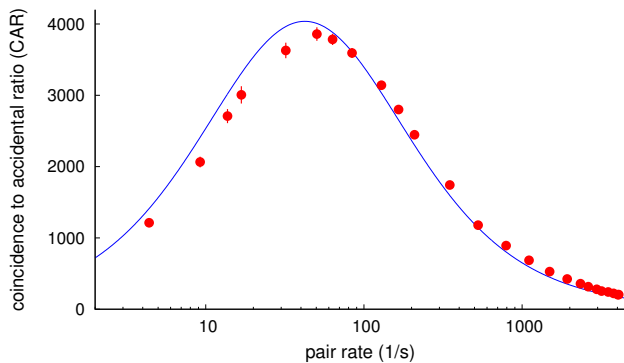
FIG. 11: The coincidence to accidental ratio (CAR) as a function of pair rates r_p . The solid line is obtained from Eq. (14) with \eta_s = 17.3\% , \eta_i = 12.4\% , d_s = 165 \text{ s}^{-1} , d_i = 508 \text{ s}^{-1} , \Delta t = 30 ns.
