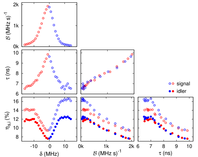
FIG. 14: Summary of the effect of two-photon detuning \delta on heralding efficiencies \eta_{s,i} , coherence time \tau , and spectral brightness \mathcal{B} . Other parameters: P_{776} = 15 mW, P_{780} = 450 \mu W, \Delta = -60 MHz, OD=29.
