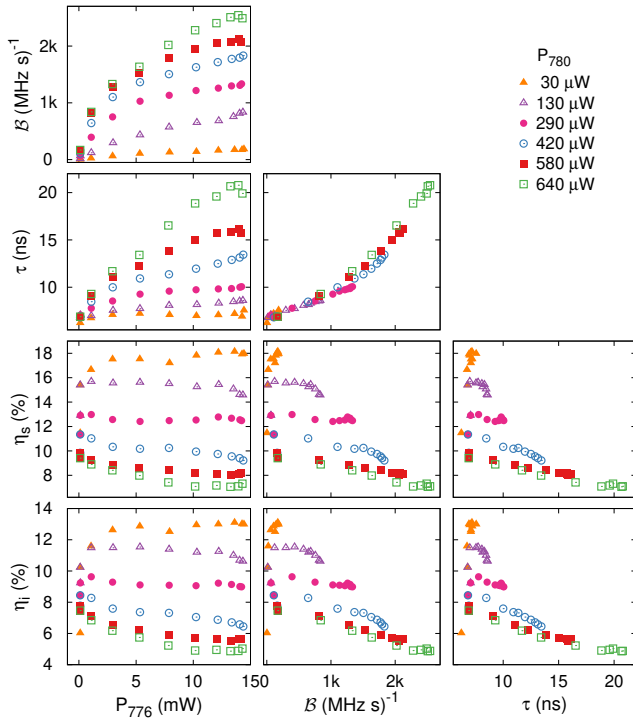
FIG. 15: Summary of the effect of pump powers P_1 and P_2 on heralding efficiencies \eta_{s,i} , coherence time \tau , and spectral brightness B . Other parameters: OD=29, \Delta = -60 MHz, \delta = 3 MHz.
