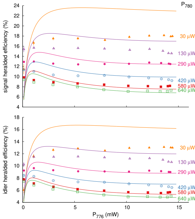
FIG. 8: heralding Heralding efficiency as function of P_{776} for the signal (top) and idler (bottom) for different P_{780} . The vertical error bar on each point is smaller than the size of the data points. Other parameters: OD=29 , \Delta = -60 MHz, \delta = 3 MHz. The solid lines are a numerical fit with Eq. 5. The model fails to describe the experimental behavior for low pump powers. As discussed in the main text, in this region the power broadening is comparable with the pump lasers linewidths, a regime beside the model assumptions.
