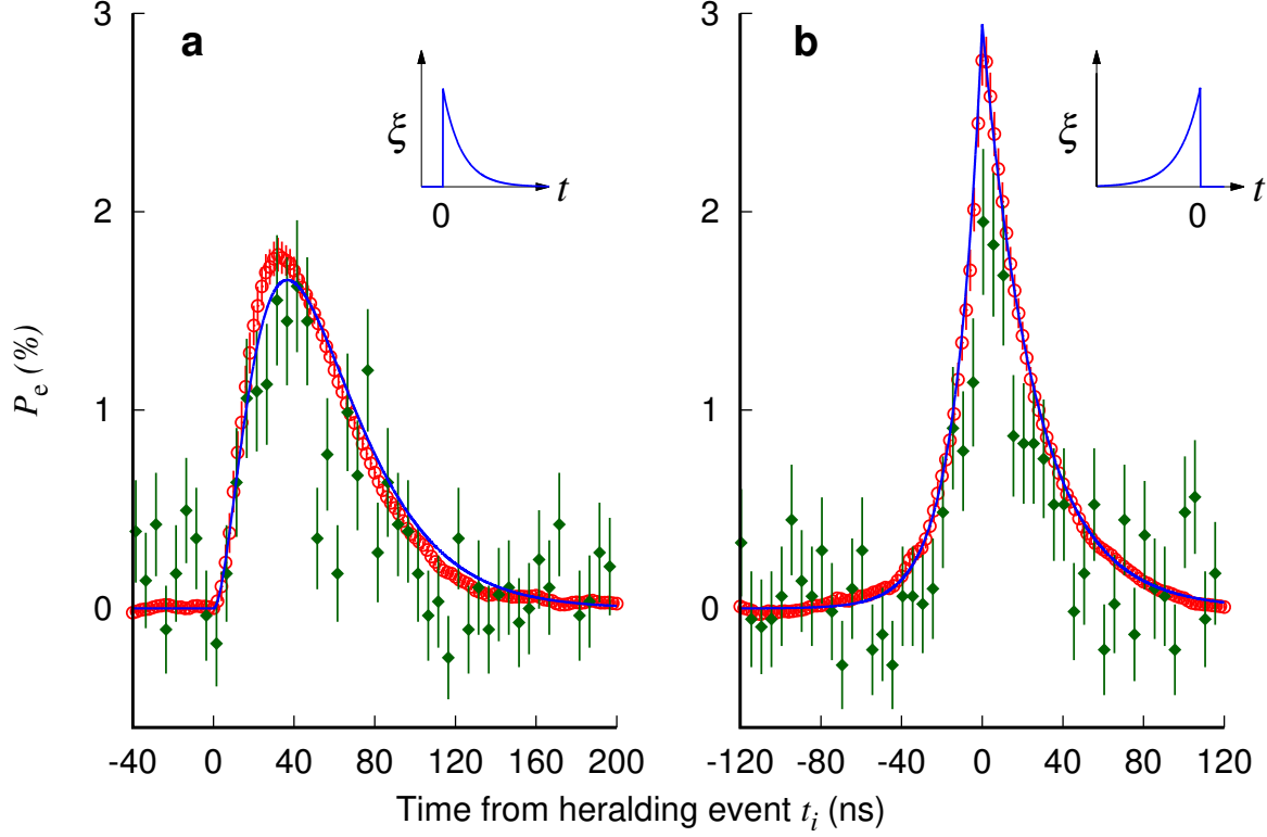
FIG. 5. Time-resolved atomic excited state population P_e . (a) Exponentially decaying and (b) exponentially rising probe photons. Red open circles, time bin size 2 ns: P_e(t_i) obtained from forward detection rates integrating Eq. 7. Error bars represent one standard deviation of the distributions obtained by a Monte-Carlo method and assuming Poissonian statistics for the detection rates. Green filled diamonds, time bin size 5 ns: P_e(t_i) obtained from the backward detection rates using Eq. 5. Error bars show one standard deviation assuming Poissonian statistics for the detection rates. Solid lines: P_e(t) from Eq. (3) and (4) using \tau_p = 13.3 ns, \Lambda = 0.033 .
