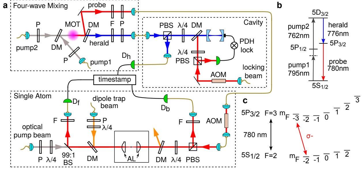
FIG. 2. Experimental setup and level schemes. (a) (Top left) Four-wave mixing part, providing heralded single photons: pump 1 (795 nm) and pump 2 (762 nm) are overlapped in a copropagating geometry inside the cold cloud of ^{87}\text{Rb} atoms in a magneto-optical trap (MOT), generating pairs of herald (776 nm) and probe (780 nm) photons. The detection of a photon at D_h heralds a probe photon. (Top right) Tuning the resonance of a bandwidth-matched cavity with respect to the heralding photon frequency controls the temporal envelope. (Bottom) Single atom part: A ^{87}\text{Rb} atom is trapped at the focus of a confocal aspheric lens pair (AL; numerical aperture 0.55) with a far-off-resonant optical dipole trap (980 nm). The probe photons are guided to the single atom part by a single mode fiber and focused onto the atom by the first AL. Avalanche photodetectors D_f and D_b detect photons collected in forward and backward directions. An acousto-optic modulator (AOM) shifts the probe photon frequency to compensate for the shift of the atomic resonance frequency caused by the bias magnetic field and the dipole trap. D_h , D_f , D_b : avalanche photodetectors (APDs), P: polarizer, F: interference filter, \lambda/2 , \lambda/4 : half- and quarter-wave plates, (P)BS: (polarizing) beam splitter, DM: dichroic mirror, PDH lock: Pound-Drever-Hall frequency lock electronics. (b) Relevant level scheme of the four-wave mixing process in a cloud of ^{87}\text{Rb} atoms. (c) Relevant level scheme of the single ^{87}\text{Rb} atom in the dipole trap. The probe photons are resonant with the closed transition |g\rangle = 5S_{1/2}, F=2, m_F=-2 to |e\rangle = 5P_{3/2}, F=3, m_F=-3 .
