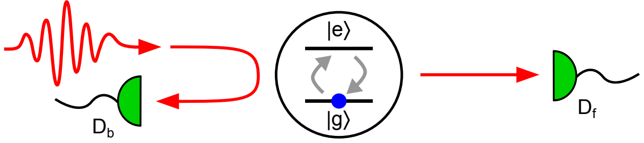
FIG. 1. Single photon scattering by a two-level atom in free-space. The time evolution of the atomic excited state population is inferred by measuring photons in the forward or backward direction. D_f and D_b : forward and backward detectors, |g\rangle and |e\rangle : ground and excited levels of the atom.
