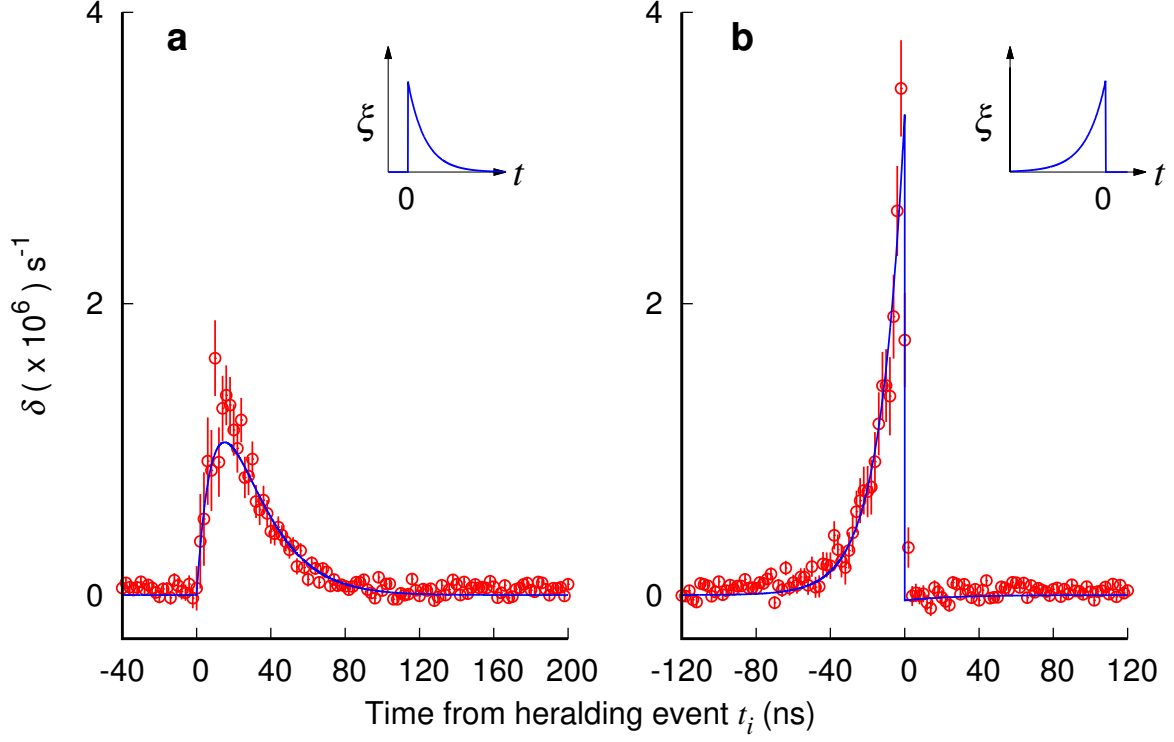
FIG. 4. Time-resolved changes in single-photon transmission rates. Changes in the forward detection rates \delta(t_i) = R_{f,0}(t_i) - R_f(t_i) induced by the interaction with the atom for exponentially decaying (a) and rising (b) probe photons. The time bin size is 2 ns. Solid lines: analytical solution of Eq. 6 using Eq. (1,2, and 3) for \tau_p = 13.3 ns, \Lambda = 0.033 . Error bars represent one standard deviation, assuming Poissonian statistics for R_{f,0}(t_i) and R_f(t_i) .
