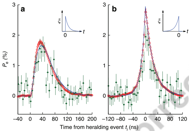
Figure 5 | Time-resolved atomic excited state population P_e .
