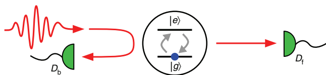
Figure 1 | Single photon scattering by a two-level atom in free space.
