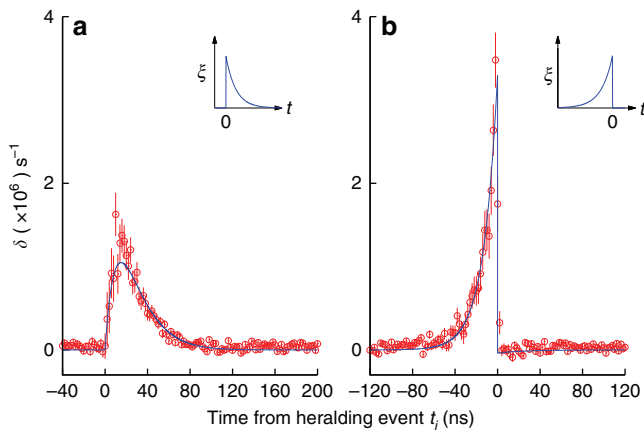
Figure 4 | Time-resolved changes in single-photon transmission rates.
