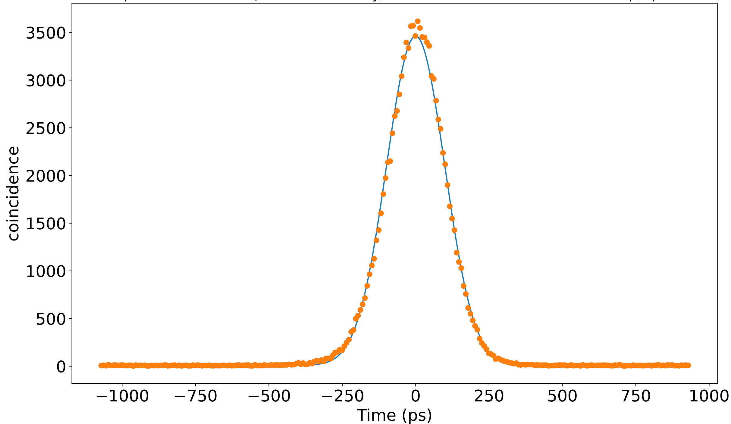
1550nm pair source with 2 IDQubes 30% efficiency, 10us dead time with non-blue timestamp, 8ps time bin
