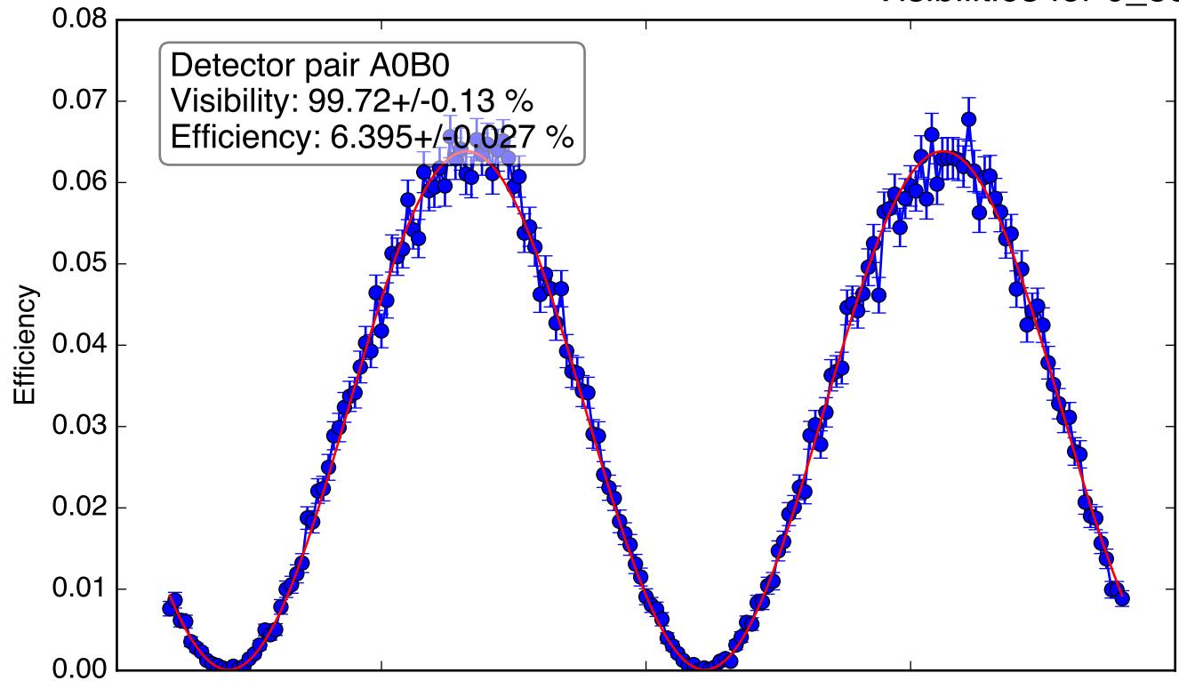
Visibilities for 0_8594_20141021.dat
