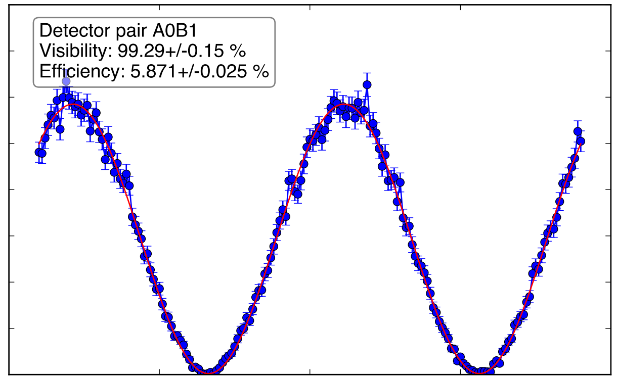
Visibilities for 0_8594_20141021.dat
