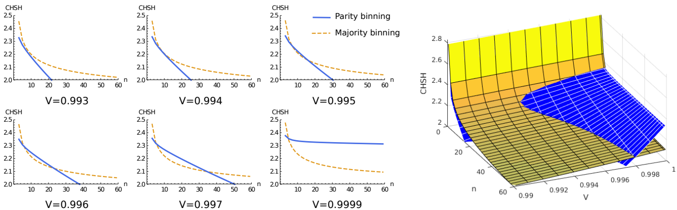
FIG. 7. CHSH violation achieved by the majority and parity binnings as a function of the source visibility V and number of pairs n . For V \lesssim 0.994 , the largest Bell violation is achieved by the majority strategy. For V \gtrsim 0.994 , the parity strategy provides a large violation for a range of n .
