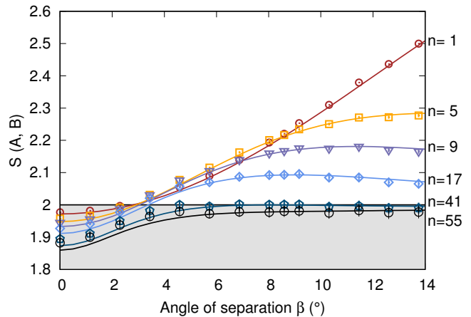
FIG. 4. Majority processing for different n applied to the data. The error bars are obtained from the bootstrapping procedure indicated in the text. The continuous lines are obtained numerically following section II B, with V = 0.9892 .
