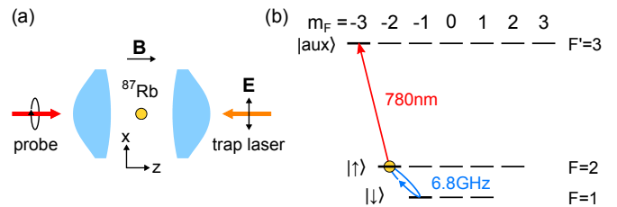
FIG. 1: (a) Simplified optical setup. A single atom is held by a linearly polarized FORT and is probed with a circularly polarized beam. (b) Energy level scheme. The two 5S_{1/2} Zeeman levels |F = 2, m = -2\rangle \equiv |\uparrow\rangle and |F = 1, m = -1\rangle \equiv |\downarrow\rangle are used as qubit states. The |\uparrow\rangle state is coupled via a closed optical transition to the 5P_{3/2} |F' = 3, m = -3\rangle \equiv |\text{aux}\rangle state.
