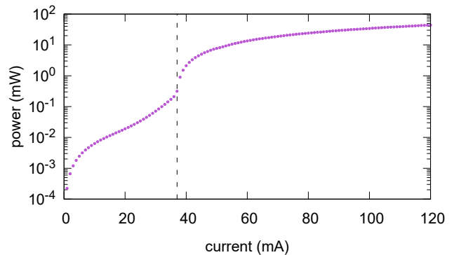
FIG. 4. Measured laser power against laser current I_L . The sharpest change is observed at I_T = 37 mA, indicating the threshold current (dashed line).
