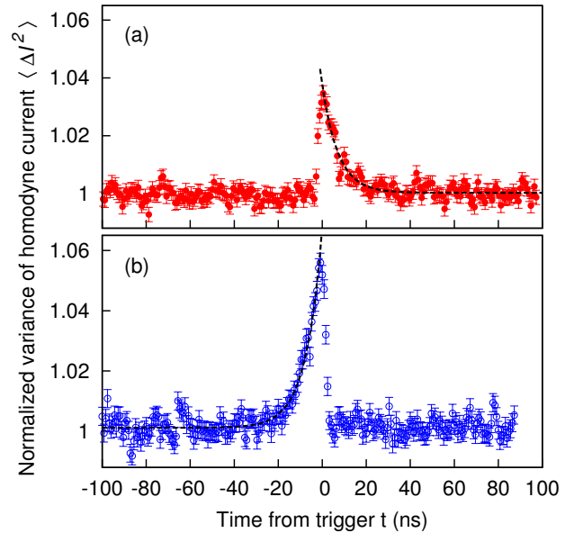
FIG. 4: (Color online) Optical homodyne results. (a) Exponential decay of the field variance of heralded idler photons. (b) Exponential rise of the field variance of heralded signal photons.
