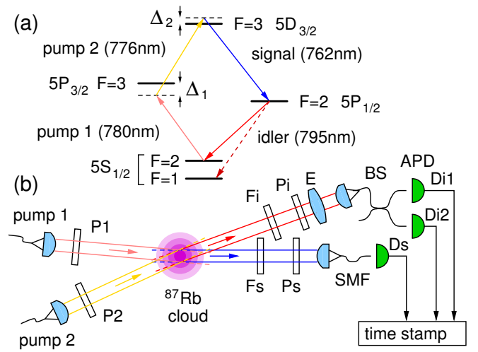
FIG. 1: (Color online)(a) Cascade level scheme for four wave mixing in ^{87}\text{Rb} . (b) Setup of the heralded single photon source. Polarizers (P1,2, Pi, Ps) and interference filters (Fi, Fs) separate the signal and idler photons from residual pump light. An etalon (E) in the idler arm removes uncorrelated photons from a decay to the 5S_{1/2}, F=1 level. Signal photons detected by an avalanche photodiode (APD) trigger a Hanbury-Brown–Twiss measurement between idler photons distributed to two detectors, D_{i1} and D_{i2} , via a 50:50 fiber beam splitter (BS).
