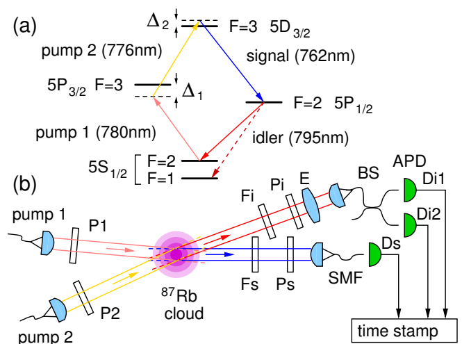
FIG. 1: (Color online) (a) Cascade level scheme for four wave mixing in ^{87}\text{Rb} . (b) Setup of the heralded single photon source. Polarizers (P1,2, Pi, Ps) and interference filters (Fi, Fs) separate the signal and idler photons from residual pump light. An etalon (E) in the idler arm removes uncorrelated photons from a decay to the 5S_{1/2}, F = 1 level. Signal photons detected by an avalanche photodiode (APD) trigger a Hanbury-Brown-Twiss measurement between idler photons distributed to two detectors, D_{i1} and D_{i2} , via a 50:50 fiber beam splitter (BS).
