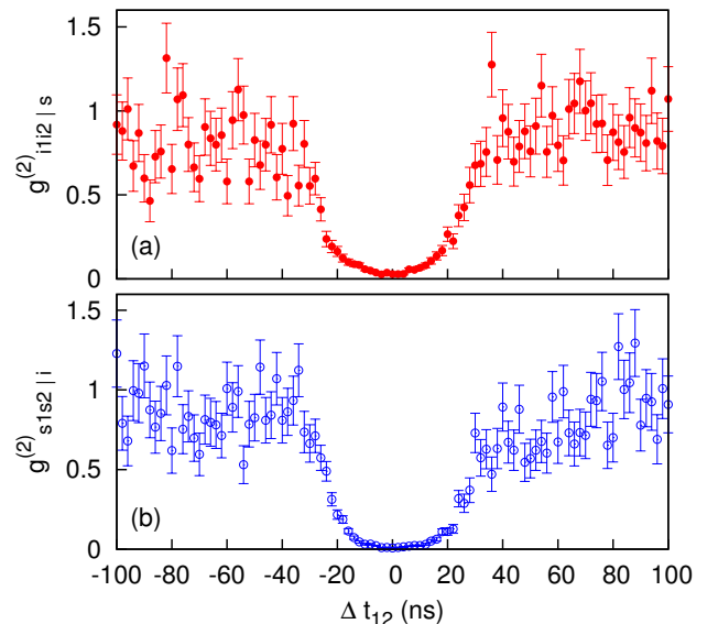
FIG. 2: (Color online) (a) The correlation function g_{i1i2|s}^{(2)} of idler photons separated by a time difference \Delta t_{12} , conditioned on detection of a heralding event in the signal mode, shows strong photon antibunching over a time scale of \pm 20 ns, indicating the single photon character of the heralded photons. The error bars indicate the propagated poissonian counting uncertainty from G_{i1i2|s}^{(2)} and N_{i1i2|s} . (b) Same measurement, but with the signal and idler modes swapped.
