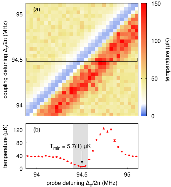
FIG. 5. (a) Atomic temperature for various probe and coupling field detunings, inferred from release and recapture measurements after 20 ms of EIT cooling. The anti-diagonal blue band indicates dark state resonance which has the highest cooling efficiency. (b) EIT cooling profile in atomic temperature as a function of probe detuning \Delta_p for a fixed coupling detuning (here \Delta_c = 2\pi \times 94.5 MHz as indicated by the boxed region in (a)) also shows an asymmetric Fano feature. The area shaded in gray represents the range of probe detunings where an effective cooling is observed.
