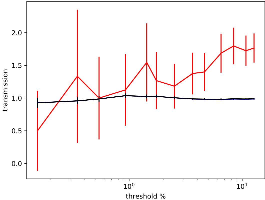
postselected transmission
