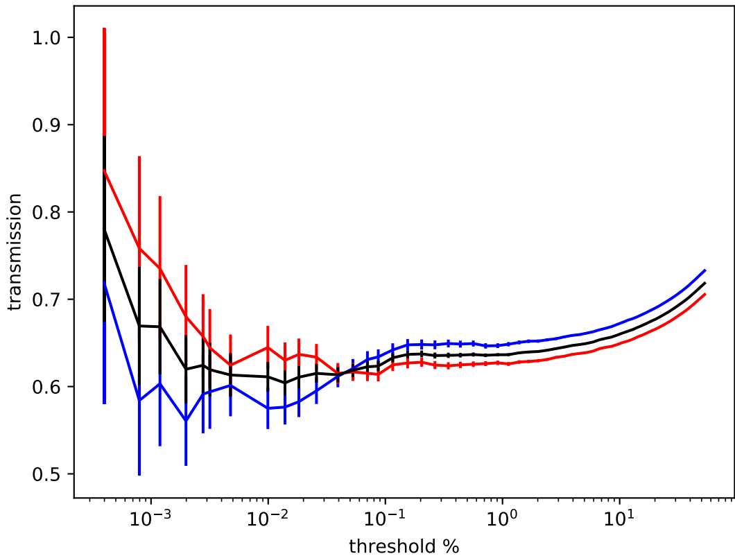
postselected transmission
