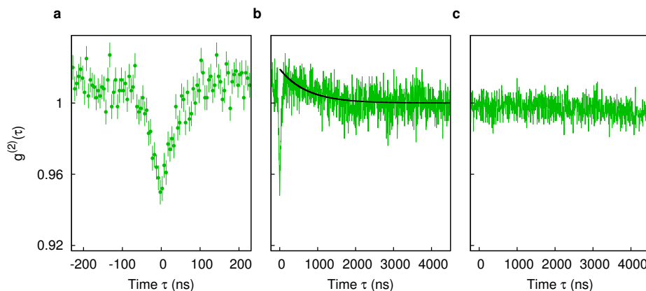
FIG. 8. Photon bunching due to atomic motion. a , Normalized second order correlation function without deconvolution of the diffusive atomic motion. b , Same as a but with extended range. Solid line is a fit to f(\tau) = 1 + a_0 \exp(-\tau/\tau_d) with a_0 = 0.019(2) , \tau_d = 0.71(8) \mu\text{s} and a reduced \chi^2 = 1.07 . c , Same as b but computed from events during the reference cycle, i.e., when the atom is not resonant with probe field.
