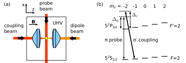
FIG. 4. (a) Experimental configuration for the off-resonant EIT cooling process. The probe beam propagates orthogonally to the optical axis to allow for motional coupling. (b) Energy levels and transitions in ^{87}\text{Rb} used in the cooling experiment.
