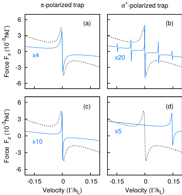
FIG. 2: Calculated force on an atom of fixed velocity moving through a \sigma^+-\sigma^- PGC field for different axes and FORT polarizations. Both beams of the PGC field have a Rabi frequency \Omega = \Gamma_0/2 and are red-detuned from the natural transition frequency by \Delta = -3\Gamma_0 , where \Gamma_0 = 2\pi \times 6.07 MHz is the natural linewidth. Black dashed and blue solid lines indicate the force for a free and a trapped atom, respectively. (a) \pi -polarized trap, PGC field along x axis. (b) \sigma^+ -polarized trap, PGC field along x axis. (c) \pi -polarized trap, PGC field along z axis. (d) \sigma^+ -polarized trap, PGC field along z axis.
