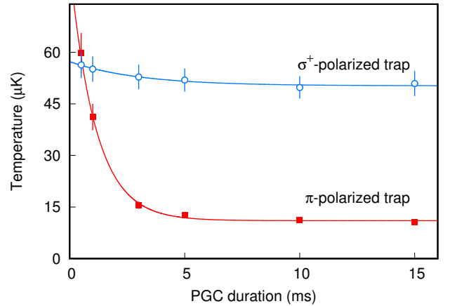
FIG. 5: Temperature of the atoms after PGC for a varying cooling duration. Optimal cooling beam power is used respectively for both the \pi -polarized trap (red square) and the \sigma^+ -polarized trap (blue circle). Solid lines are fits to exponentials. Error bars represent one standard deviation.
