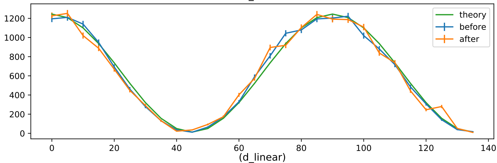
Visibility Curves Before vs After circulator (v_linear)
