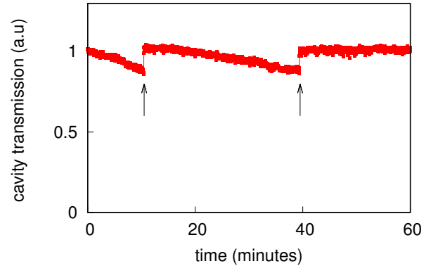
FIG. 6: Transverse stability of the near-concentric cavity at the last stable longitudinal resonance ( d = 207 nm). The slow drift of cavity transmission on the order of minutes is due to the transverse misalignment caused by temperature change, while the cavity length is locked to a probe light resonance during the measurement. Vertical arrows indicate the activation of the stabilization algorithm, where the cavity transmission recovers to the maximum value after the successful implementation of the algorithm within a few seconds.
