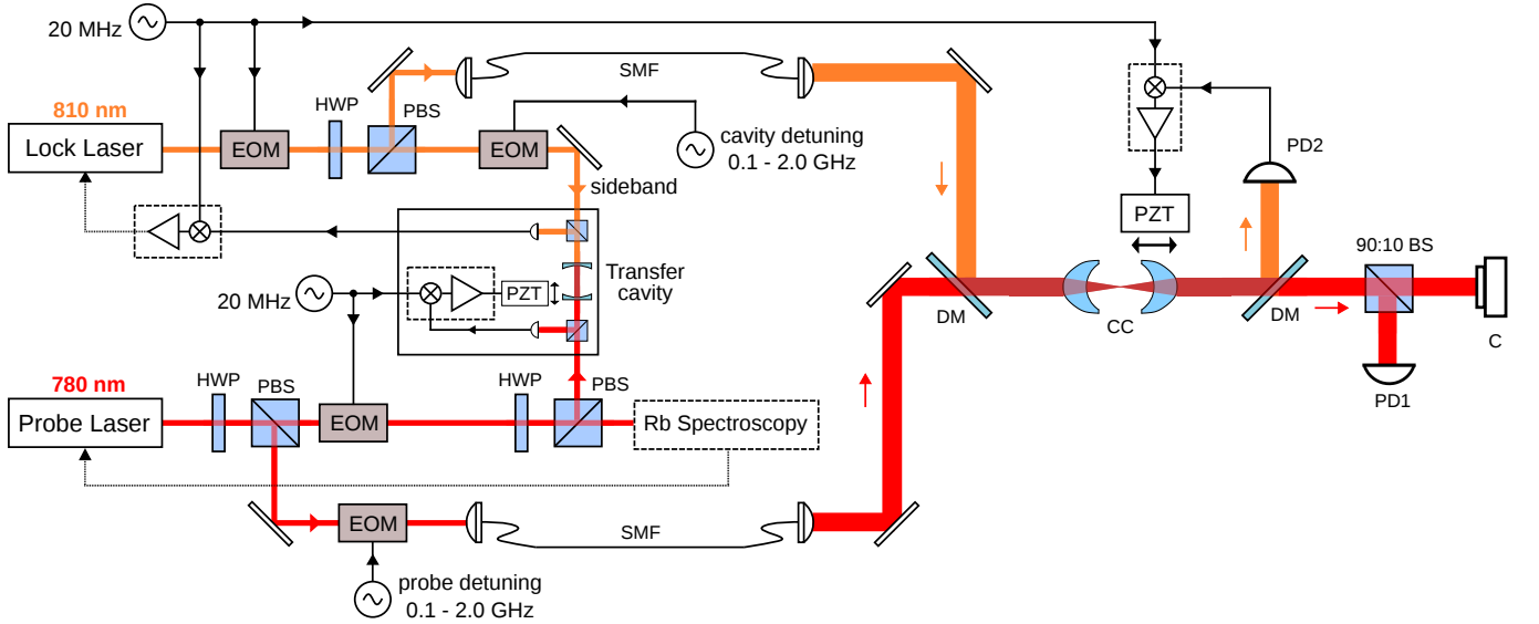
FIG. 2: Locking scheme of the near-concentric cavity setup. Red and orange lines indicate the beams from 780 nm probe laser and 810 nm lock laser, respectively. The frequency of the probe laser is stabilized to a D2 transition of ^{87}\text{Rb} by modulation transfer spectroscopy. The lock laser's sideband is locked to resonance of the transfer cavity, which in turn is stabilized to the probe laser. The frequency of the lock laser can be tuned by adjusting the sideband frequency. The near-concentric cavity is stabilized to the lock laser. All cavity locking schemes use the standard Pound-Drever-Hall technique with 20 MHz phase modulation. The cavity transmission of probe and lock lasers are separated by a dichroic mirror (DM). A camera with linear response (C) and a photodetector (PD1) are placed at the cavity transmission's 780 nm arm to observe the resonant modes. PBS: polarization beam splitter. BS: beam splitter. SMF: single-mode fibers.
