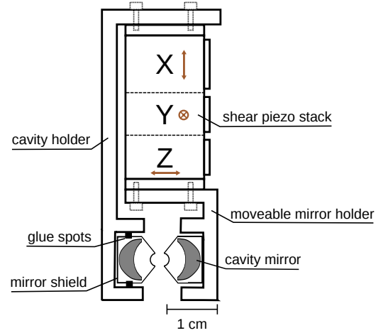
FIG. 1: Schematic of a near-concentric cavity assembly. Arrows indicate the moving directions of piezo segments.
