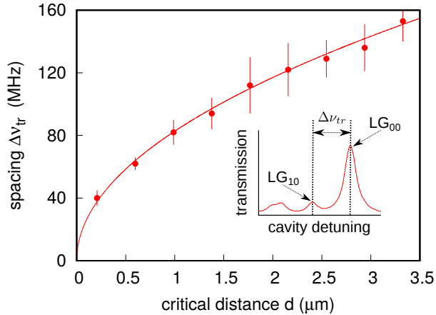
FIG. 3: Transverse-mode frequency spacing ( \Delta\nu_{tr} ) at different critical distance ( d ) of cavity lengths that are resonant with 780 nm laser. The solid line is the fit based on Eq. 2. Error bars show the standard deviation of the measurement. The inset shows a typical cavity transmission spectrum and the derived \Delta\nu_{tr} .
