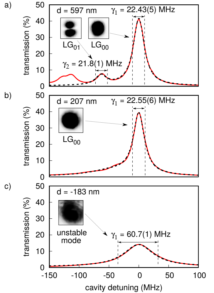
FIG. 4: Cavity transmission spectra, measured by detuning the cavity through small changes (few nm) in the cavity length. (a) d = 597 nm. The dashed line is a fit to a sum of two Lorentzian functions modeling two resonant peaks. (b) d = 207 nm. Transverse modes become degenerate and form a long tail extending out to the lower frequencies. (c) d = -183 nm. The cavity is in the unstable regime. Insets show the transmitted transverse mode profiles recorded by a (partly saturated) camera.
