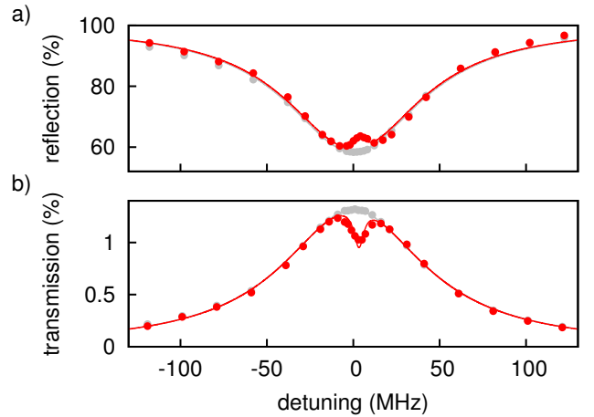
FIG. 4: Onset of the normal-mode splitting in the a) reflection and b) transmission spectrum when an atom is trapped in the FORT. Red solid lines are fits based on Eq. 7. For comparison the empty cavity reflection/transmission (Fig. 2a) is shown in gray.
