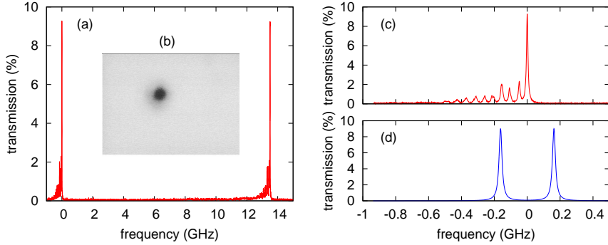
Figure 7. (a) Measured transmission through an anaclastic cavity for the cavity length 780 nm away from the concentric configuration, and an input beam waist \omega=3.6 mm corresponding to a focusing parameter u = 0.36 . Inset (b) shows that the spatial mode profile for the fundamental transverse mode (largest transmission), recorded with a camera chip after demagnification with a converging lens. Part (b) shows a zoom into the transmission structure, where residual excitation of higher spatial modes can be resolved due to imperfect mode matching. Panel (d) shows the simulated normal mode splitting we would expect for these cavity parameters from a single Rb atom, assuming no higher spatial modes are present.
