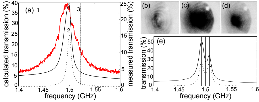
Figure 5. The effect of the aberrations in the cavity transmission spectrum. a) The measured spectrum (red line) and the calculated spectrum (black solid line) of cavity transmission with a focusing parameter of 0.047 are compared. The calculated fundamental mode of the cavity is also shown as a reference (dashed line). The vertical lines 1,2 and 3 (in a) are the frequency references of the snapshots of the cavity transmission b,c and d, respectively. The detection area of the camera is 3 \times 4 \text{ mm}^2 and the images are in real dimensions of the chip size of the camera. e) Normal mode splitting of the calculated transmission at focusing parameter of 0.047, where the coupling coefficient g_0 is 7.75 MHz (solid line). The vertical lines show the frequencies of the splitted modes and the cavity resonance. The normal mode splitting of the fundamental mode of the cavity is also shown as a reference (dashed line).
