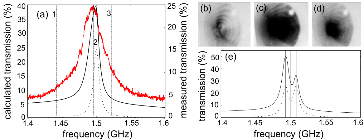
Figure 5. The effect of the aberrations in the cavity transmission spectrum. (a) The measured spectrum (red line) and the calculated spectrum (black solid line) of cavity transmission with a focusing parameter of 0.047 are compared. The calculated fundamental mode of the cavity is also shown as a reference (dashed line). The vertical lines 1, 2 and 3 (in (a)) are the frequency references of the snapshots of the cavity transmission (b), (c) and (d), respectively. The detection area of the camera is 3 \times 4 \text{ mm}^2 and the images are in real dimensions of the chip size of the camera. (e) Normal-mode splitting of the calculated transmission at focusing parameter of 0.047, where the coupling coefficient g_0 is 7.75 MHz (solid line). The vertical lines show the frequencies of the split modes and the cavity resonance. The normal-mode splitting of the fundamental mode of the cavity is also shown as a reference (dashed line).
