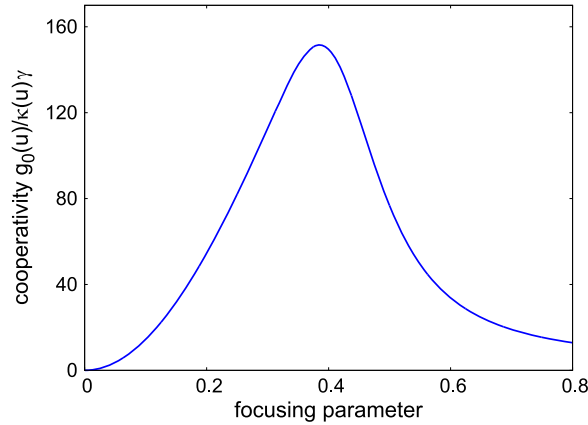
Figure 9. Estimated single atom cooperativity as a function of the focusing parameter for the anaclastic cavity coupled to a D2 transition in ^{87}\text{Rb} .
