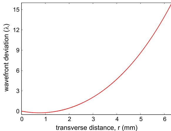
Figure 4. Aberrations in input mode at mirror. Deviation of the wavefront of the input mode from the spherical shape of the mirror surface ( R = 50 mm) as a function of transverse distance from the optical axis (in fractions of wavelength).
