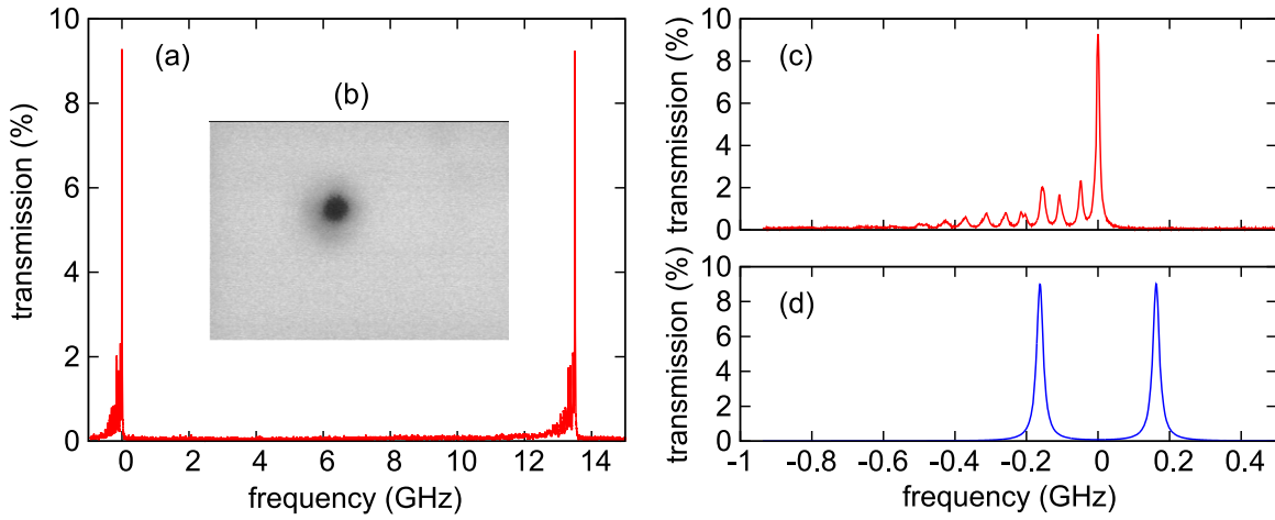
Figure 7. (a) Measured transmission through an anaclastic cavity for the cavity length 780 nm away from the concentric configuration, and an input beam waist \omega = 3.6 mm corresponding to a focusing parameter u = 0.36 . Inset (b) shows that the spatial mode profile for the fundamental transverse mode (largest transmission), recorded with a camera chip after demagnification with a converging lens. Part (b) shows a zoom into the transmission structure, where residual excitation of higher spatial modes can be resolved due to imperfect mode-matching. Panel (d) shows the simulated normal mode splitting we would expect for these cavity parameters from a single Rb atom, assuming no higher spatial modes are present.
