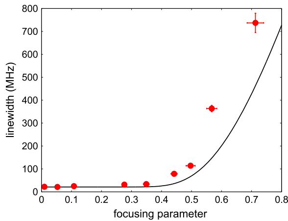
Figure 8. Measured transmission linewidth of the anaclastic cavity for different focusing parameter u (circles). The solid line represents a simulation taking into account diffraction loss only.
