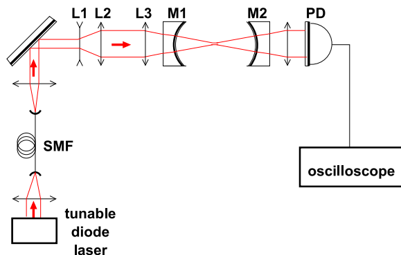
Figure 1. Experimental setup with a test cavity formed by two plano-concave mirrors M1, M2 with 0.978 reflectivity, 50 mm radius of curvature and 6.35 mm aperture. L1, L2, L3—spatial mode-matching optics, SMF—single-mode fiber for 780 nm beam and PD—photodiode.
