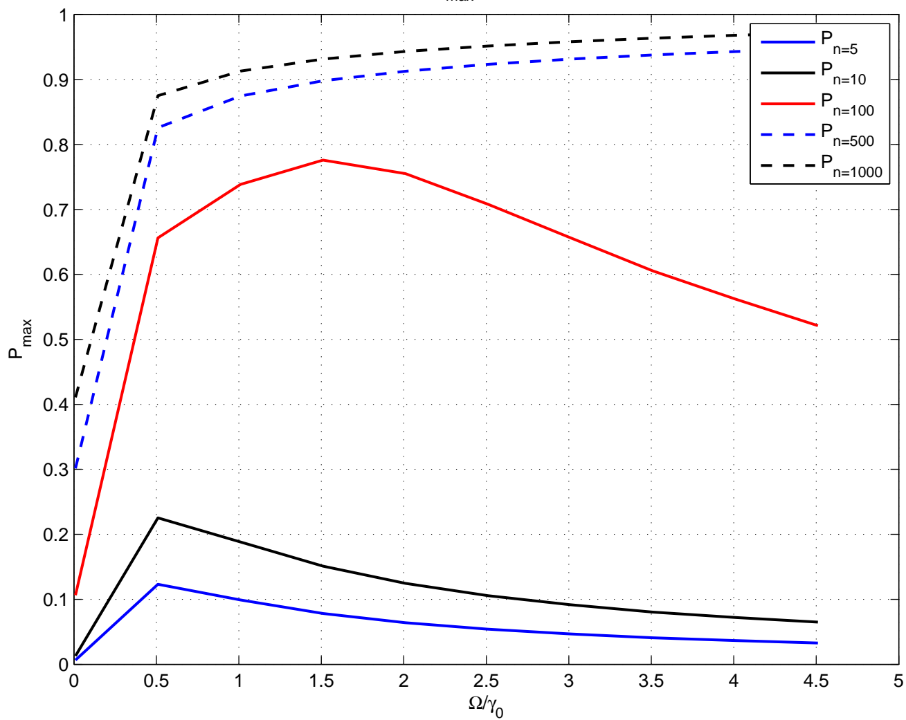
P_{\max} VS \Omega/\Gamma
